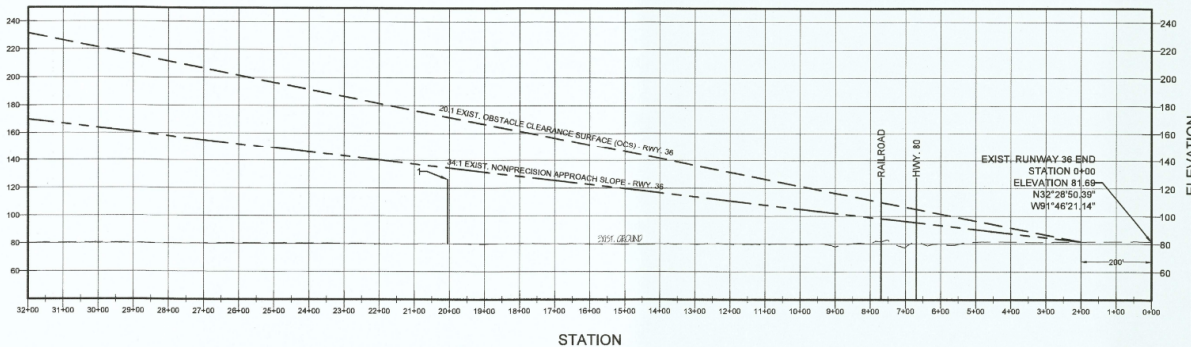
RUNWAY 36 RPZ PROFILE SCALE: HORIZ. 1"=200' VERT. 1"=50'
